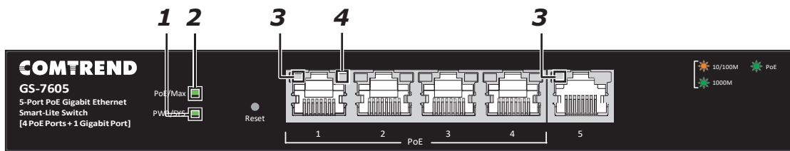
Figure 8 - GS-7605 LED Indicators
